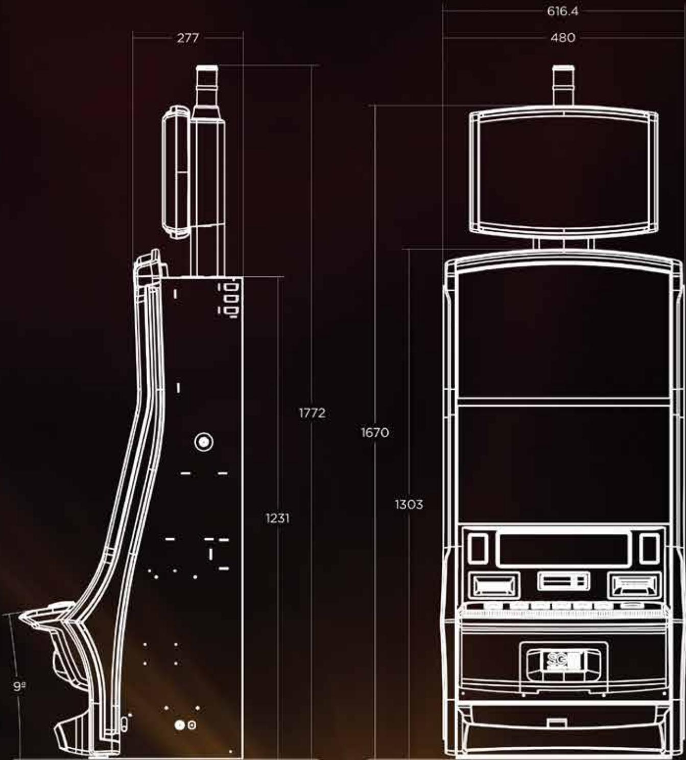
Dimension in mm
